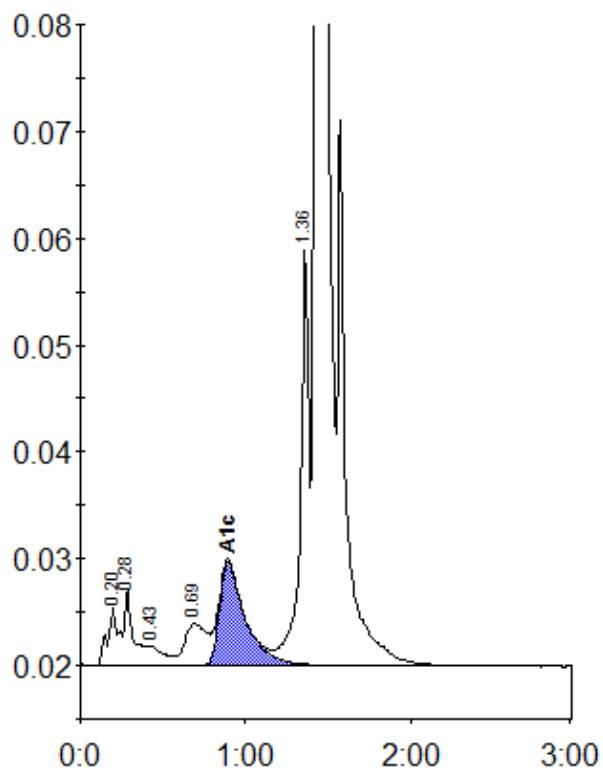
Peak table - ID: 10484816
